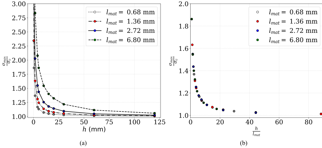
Figure 7: Maximum flexural stress to strength ratio for several (\mathcal{G}_c, \sigma_c) couples corresponding to different material characteristic lengths l_{mat} as a function of a) the specimen size and b) specimen height to material characteristic length ratio.
