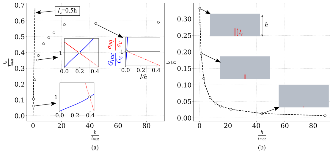
Figure 3: a) Initiation crack length to material characteristic length ratio as a function of specimen height to material characteristic length ratio. The insets show the coupled criterion in the form of stress to strength (dashed line) and incremental energy release rate to fracture toughness (thick solid line) ratios. b) Initiation crack length to specimen height ratio as a function of specimen height to material characteristic length ratio. The insets depict the size of the initiation length l_c compared to the specimen height h .
