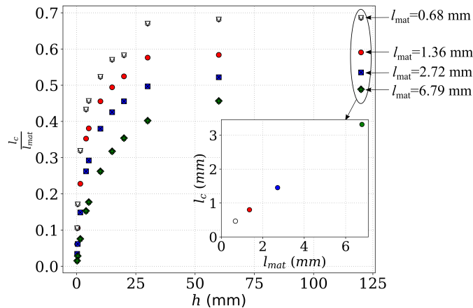
Figure 5: Initiation crack length to characteristic material length ratio as a function of the specimen size for several ( \mathcal{G}_c, \sigma_c ) couples corresponding to different material characteristic lengths l_{\text{mat}} . The inset depicts the initiation length for the largest specimen as a function of the material characteristic length.
