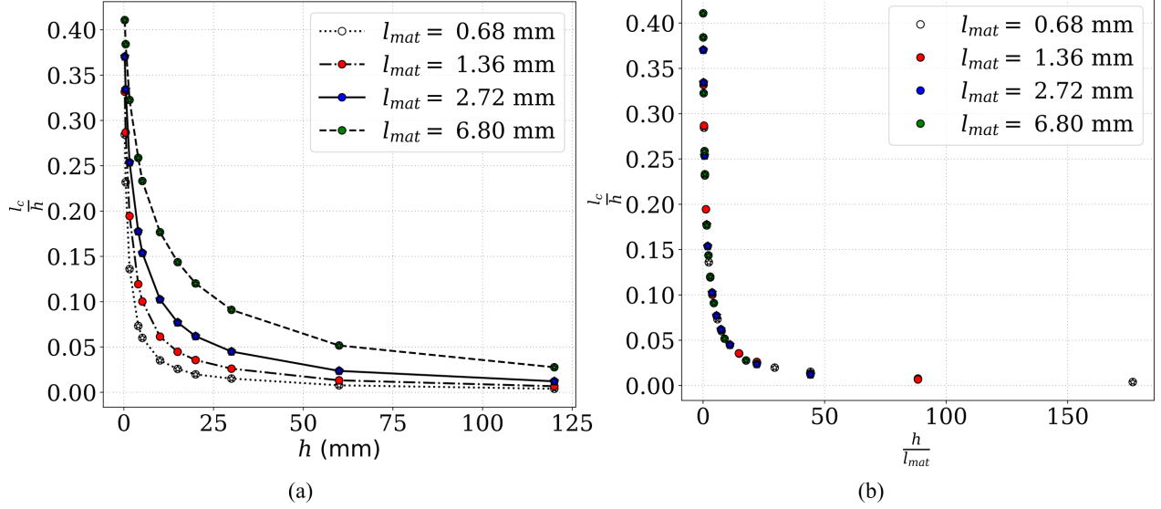
Figure 6: Initiation crack length to specimen height ratio for several ( G_c , \sigma_c ) couples corresponding to different material characteristic lengths l_{mat} as a function of a) the specimen size and b) specimen height to material characteristic length ratio.
