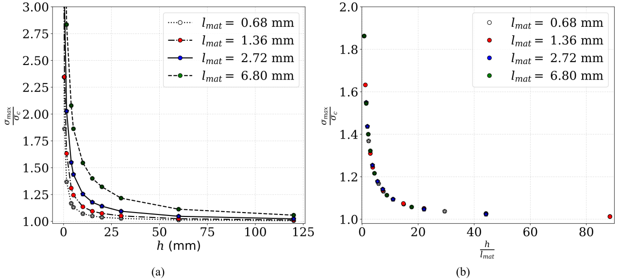
Figure 7: Maximum flexural stress to strength ratio for several ( G_c , \sigma_c ) couples corresponding to different material characteristic lengths l_{mat} as a function of a) the specimen size and b) specimen height to material characteristic length ratio.
