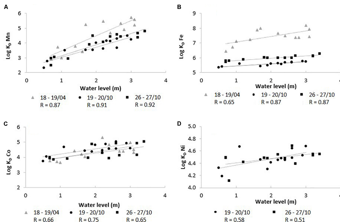
FIGURE 5 | Correlations between \text{Log } K_D of trace metals and water level for all tidal cycles in the creek during the dry (gray dots) and the wet seasons (black dots).
