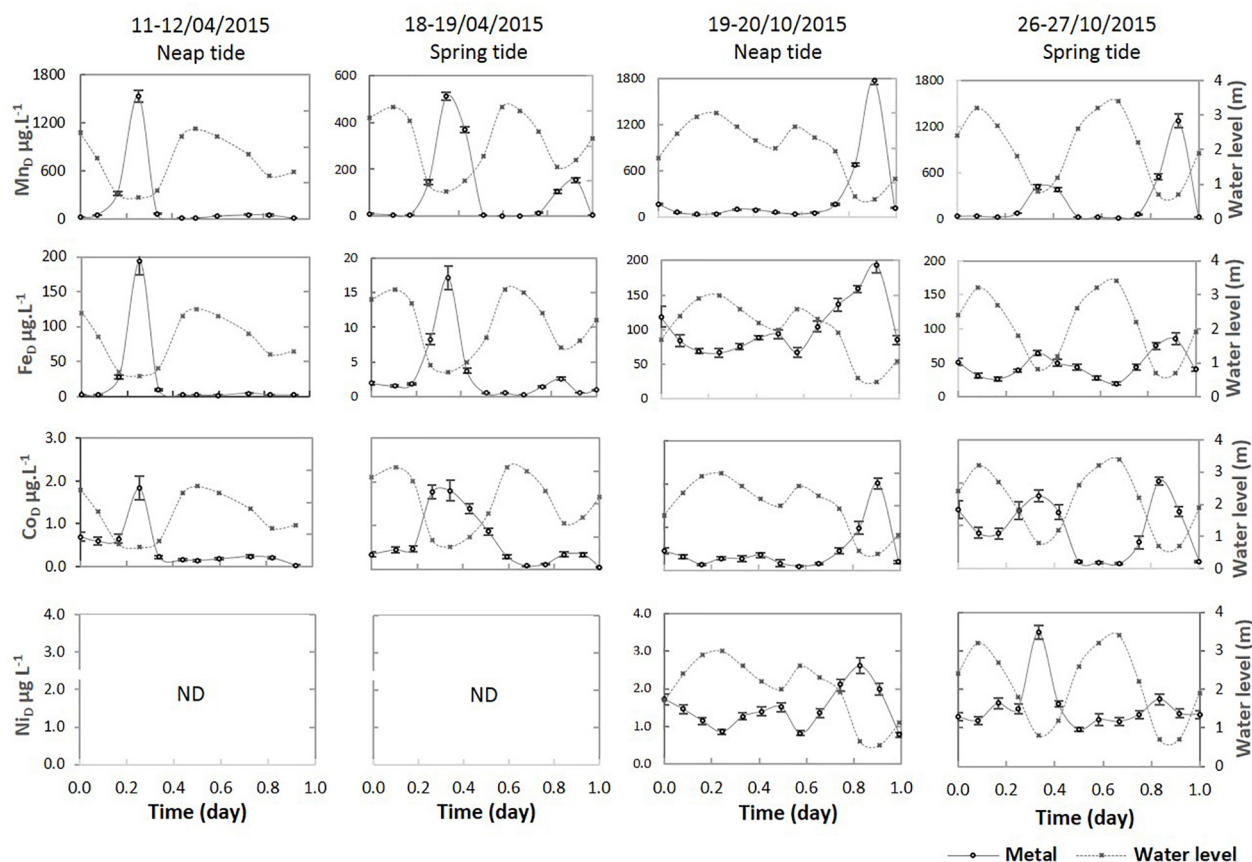
FIGURE 3 | Temporal fluctuations of dissolved metal concentrations ( M_D ) during the neap and the spring tidal cycles during the dry season (04/2015) and the wet season (10/2015). ND: not detection.
