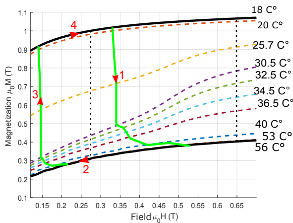
Figure 5. dashed lines: measured isothermal magnetization curves (temperature in the legend). Continuous thick lines: the working cycle taking into account the average internal field. \Delta T_{adia} = 0.2 °C and 0.1 °C during steps 2 and 4 respectively. The dotted vertical lines represent the applied fields during the steps 1 (right one at 0.65T) and 3 (left one at 0.27T)
