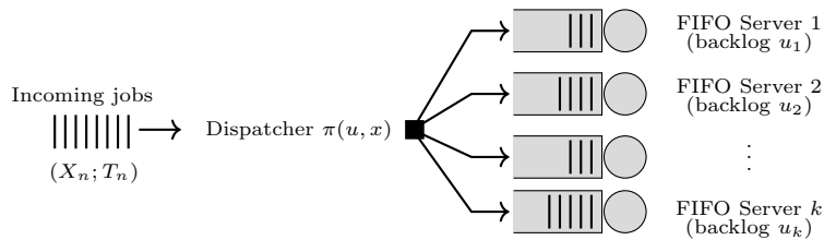
Fig. 1: Size-aware dispatching with i.i.d. service times ( X_n \stackrel{d}{=} X for all n ) and i.i.d. exponential inter-arrival times ( T_n ) to k M/G/1-FCFS servers.
