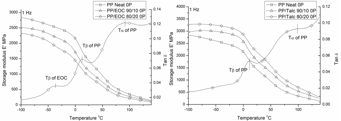
Fig.a: EOC (left) and talc (right) content effect on PP Storage modulus at 1 Hz
