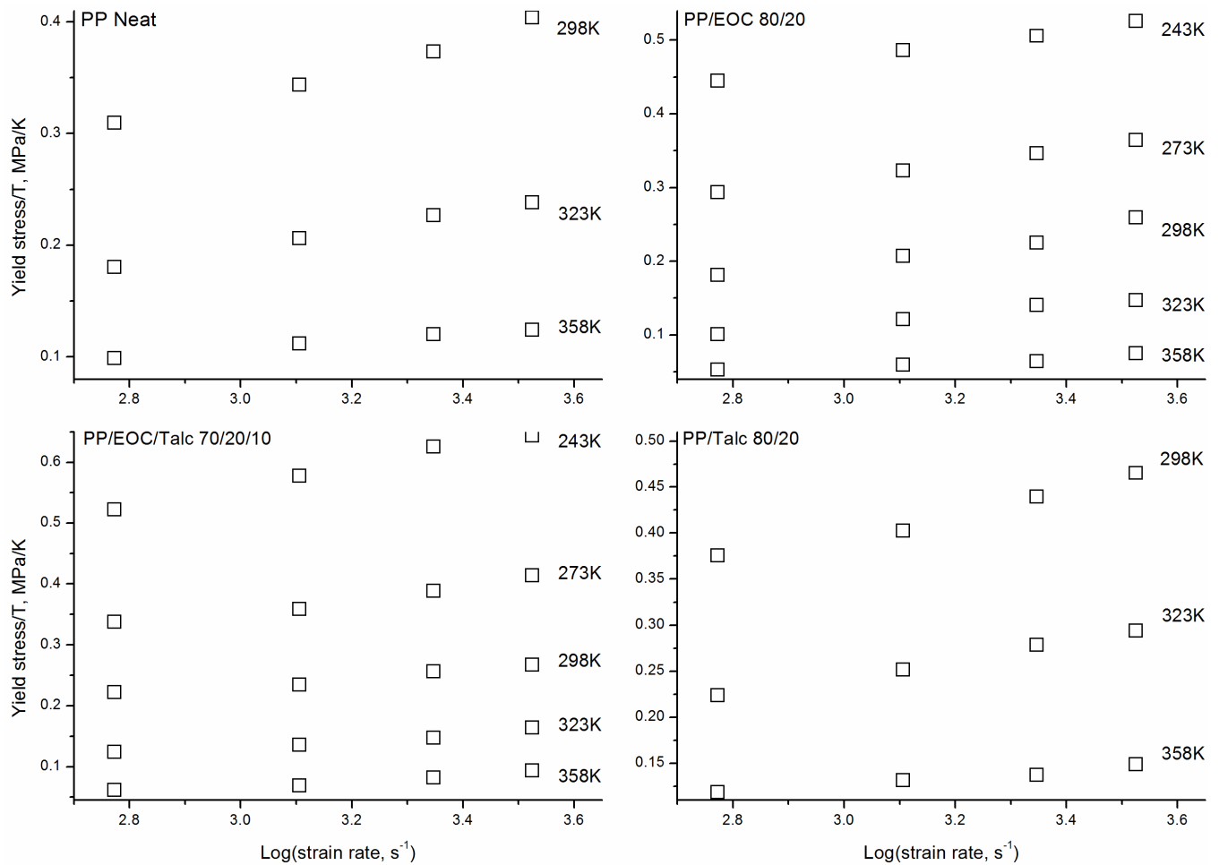
Fig. c: The dependences of yield stress in dynamic compression on strain rate and recycling number at five temperatures.
