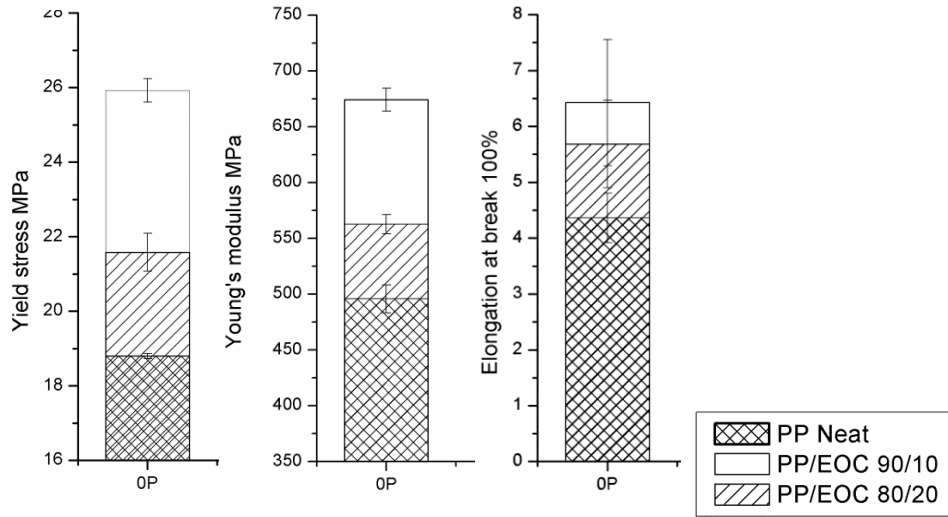
Fig.b : Elastic properties for the different filler contents for quasistatic tensile tests
