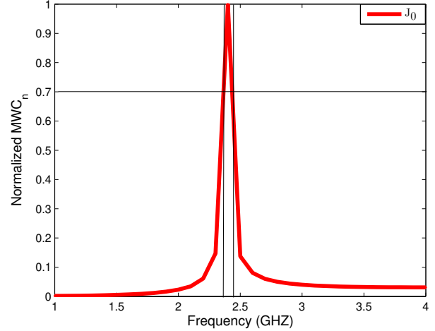
FIG. 8: Normalized MWC_n with respect to frequency of BC-SRR.
