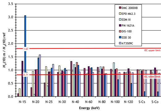
Figure 2. Energy response of APDs in continuous mode (for dose equivalent rate H_p(10) around 10 mSv.h -1 , and integrated dose equivalent around 0.5 mSv)
