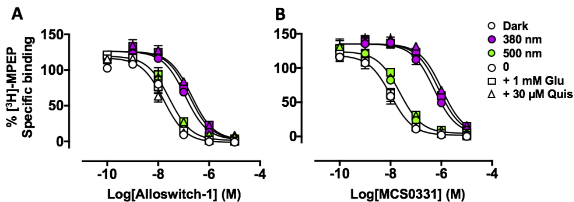
Figure 5. [ ^3\text{H} ]-MPEP competition radioligand binding studies to demonstrate the effect of either a saturating concentration of glutamate (1 mM glu) or quisqualate (30 \mu\text{M} quis) on alloswitch-1 (A) or MCS0331 (B) - mediated inhibition of [ ^3\text{H} ]-MPEP binding in hmGlu _5 expressing membranes. Data are expressed as a percentage of specific binding and represent the mean \pm SEM of at least three independent experiments performed in duplicate. Fitted curves are from global analysis of datasets according to Equation 3 (in Methods) with parameter estimates shown in text.
