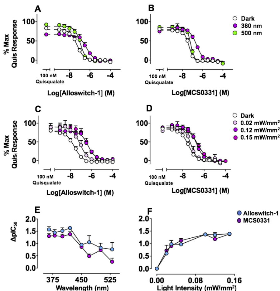
Figure 2. Effects of wavelength and irradiance on alloswitch-1 and MCS0331 negative allosteric modulation of mGlu 5 . In IP 1 accumulation assays the effect of different wavelengths of light (irradiance at 0.12 mW/mm 2 ) on the ability of alloswitch-1 (A) or MCS0331 (B) to inhibit the functioning of an EC 80 concentration of quisqualate (100 nM) was assessed at the hmGlu 5 . The ability of different irradiances of the 380 nm on alloswitch-1 (C) or MCS0331 (D) modulation of 100 nM quisqualate was also investigated. The change in pIC 50 values between dark and light conditions for each interaction was determined following illumination with different wavelengths of light (E) or illumination at 380 nm with variable irradiances (F). Data represent the mean ± SEM of at least three independent experiments performed in duplicate.
