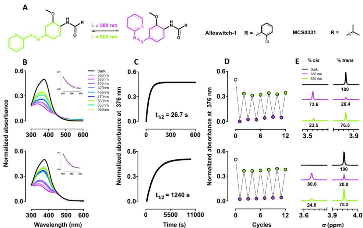
Figure 1. Chemical structure of alloswitch-1 and MCS0331 (A). UV-visible absorption spectra of 30 \mu\text{M} alloswitch-1 (B; top) and MCS0331 (B; bottom) following continuous illumination with different wavelengths of light (details in methods section) or dark conditions in 3% DMSO binding buffer, pH 7.5. Inset graphs highlights the absorption between 450 and 550 nm for alloswitch-1 (B; top) and for MCS0331 (B; bottom). Thermal relaxation of 30 \mu\text{M} alloswitch-1 (C; top) and 30 \mu\text{M} MCS0331 (C; bottom), following continuous illumination with 380 nm, in 3% DMSO, binding buffer, pH 7.5 at 37°C. Reversibility and stability of photoisomerization of 5 \mu\text{M} alloswitch-1 in binding buffer containing 5% DMSO, pH 7.5 (D; top) and 30 \mu\text{M} MCS0331 in 3% DMSO binding buffer, pH 7.5 (D; bottom) following continuous illumination with 380 nm or 500 nm. Representative ^1\text{H-NMR} spectra of (E; top) alloswitch-1 (1 mM) in DMSO- d_6 and (E; bottom) MCS0331 (500 \mu\text{M} ) in 5% DMSO- d_6 in \text{D}_2\text{O} following either dark conditions or 3 min of continuous illumination with 380 nm or 500 nm at 25°C and 12°C, respectively. All absorbance data were normalized between 0 – 0.5 (B, C, D).
