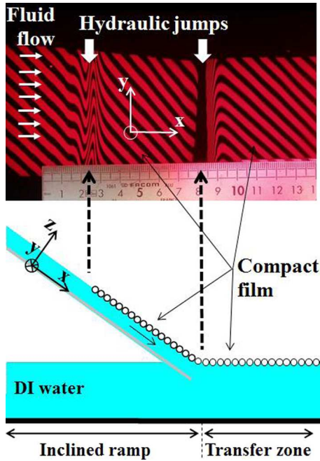
Fig. 5. Moiré pattern reflected by the moving liquid having a compact film of silica spheres floating at the surface ( \varnothing = 1 \mu\text{m} ).
