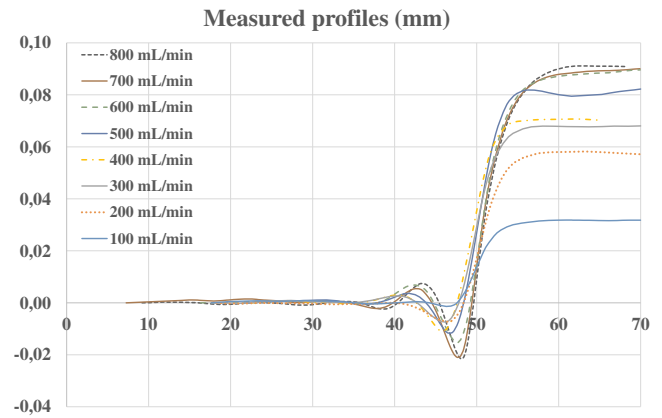
Fig. 9. 280 nm particles measured profiles vs. flow rate ( z origin = free surface).
