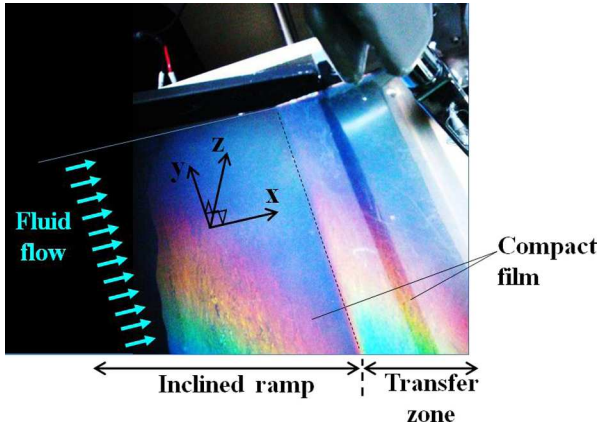
Fig. 4. Monolayer colloidal crystal of silica spheres ( \varnothing = 1 \mu\text{m} ) floating at the surface of the moving liquid (the colors arise from the diffraction of light).
