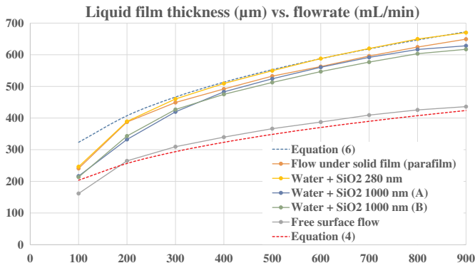
Fig. 10. Comparison between the measured film thicknesses and prediction of equations (4) and (6).
