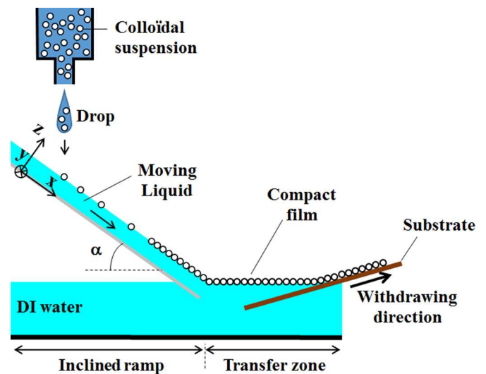
Fig. 3. Boostream ® process.
