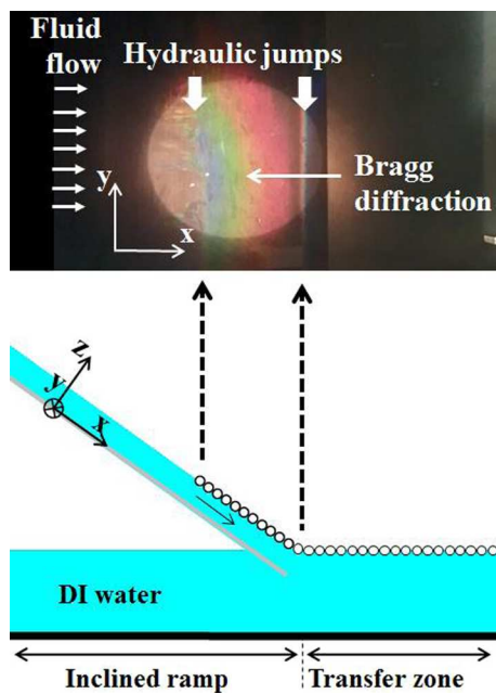
Fig. 11. View of the setup and a typical result of mode -1 of Bragg diffraction on the HCP lattice of particles.
