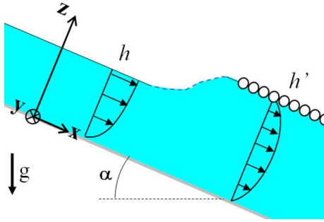
Fig. 6. Sketch of the first hydraulic jump connecting h to h' .
