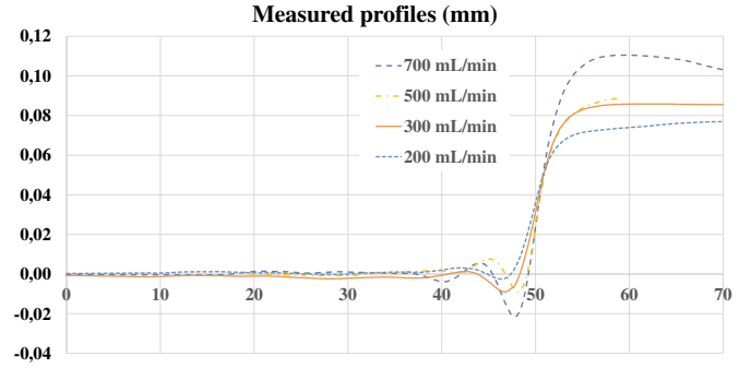
Fig. 8. 10 \mu\text{m} particles measured profiles vs. flow rate ( z origin = free surface).
