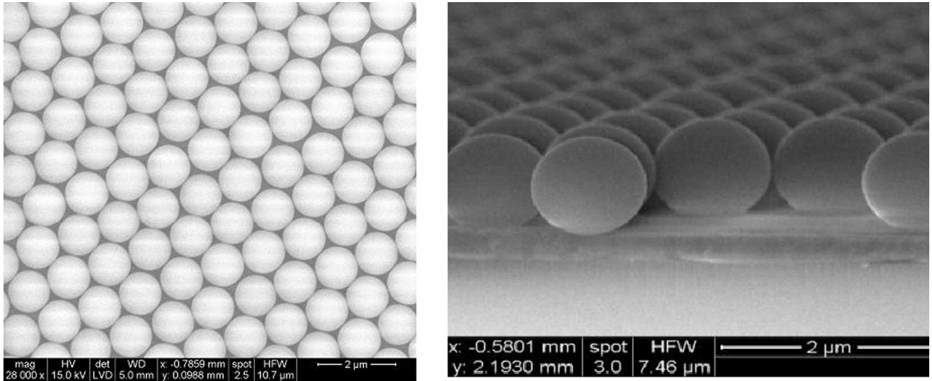
Fig. 1. SEM images of MCCs constituted of silica sphere ( \varnothing = 1 \mu\text{m} ) deposited on silicon substrate, in top view (left) and in cross section view (right).
