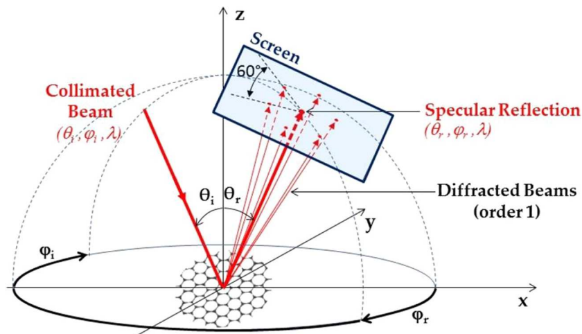
Fig. 12. Illustration of the diffraction by HCP structure at 0th and 1st order diffraction on a screen (from [12]).
