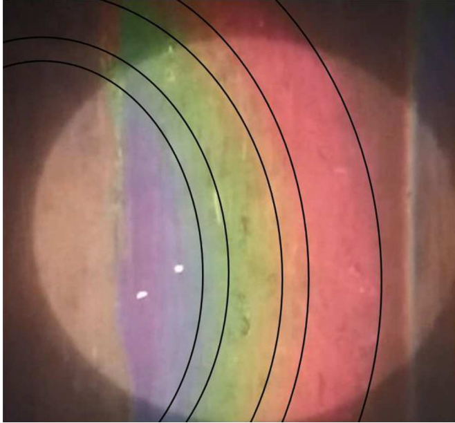
Fig. 13. Bragg diffraction on 1 \mu\text{m} particle HCP: mode -1 and extraction of isocontours for various wave lengths ( 500 \text{ mL}\cdot\text{min}^{-1} ).
