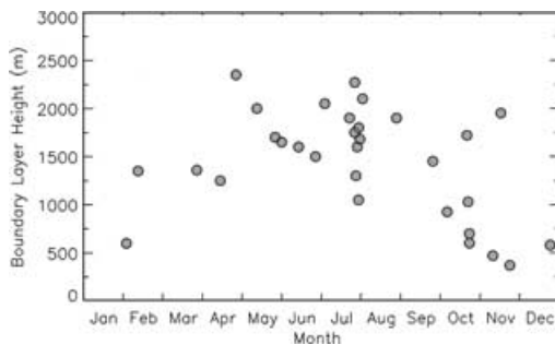
Fig. 4. Boundary layer height estimated from in-situ measurements of pressure, temperature, humidity, and CO 2 . Only mid-afternoon (12:00–17:00 LT) flights are considered.
