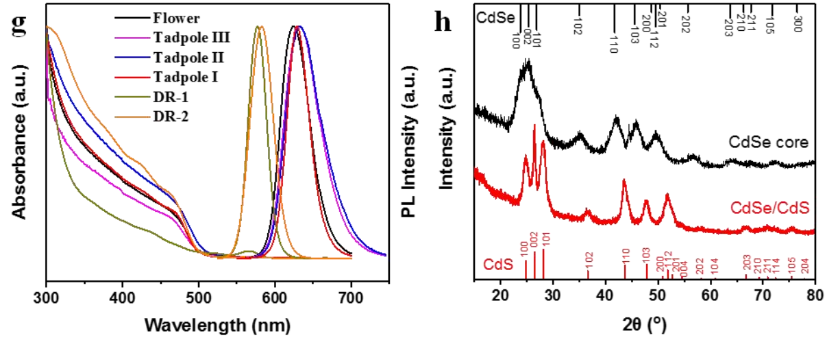
Figure 2. (a-f) TEM and high-resolution TEM (HRTEM) (insert) of CdSe/CdS NCs with different shapes: (a) nanoflowers, (b) Tadpole-III, (c) Tadpole-II, (d) Tadpole-I, (e) short dot/rods, and (f) long dot/rods. (a-2), (d-2) and (e-2) are the corresponding detailed analyses on the lattice fringes. (g) The corresponding UV-vis absorption and PL spectra, under excitation by a 450 nm
