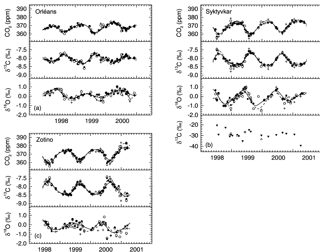
Fig. 2. (a) \text{CO}_2 mixing ratio, \delta^{13}\text{C}\text{--CO}_2 and \delta^{18}\text{O}\text{--CO}_2 observed in aircraft samples over Orléans, France ( 1^\circ\text{E} , 48^\circ\text{N} ) at three height levels, 2000 m (crosses), 2500 m (open circles) and 3000 m (closed circles). Dashed lines are harmonic fit curves through the 2000 m data, solid lines harmonic fit curves through the 3000 m data. (b) Same as (a) but for the Russian site Syktyvkar ( 52^\circ\text{E} , 61^\circ\text{N} ). The lowest panel shows apparent source signatures calculated from individual profiles where \text{CO}_2 gradients between 3000 m and 2000 m (closed symbols) and 2500 m (open symbols) were larger than 1 ppm. (c) Same as (a) but for the Siberian site Zotino ( 89^\circ\text{E} , 61^\circ\text{N} ).
