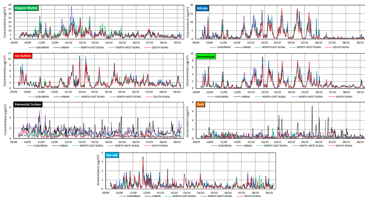
Fig. 10. Daily mass concentrations (µg m -3 ) of the major chemical compounds of fine aerosol at the five sites from 11 September 2009 to 10 September 2010.
