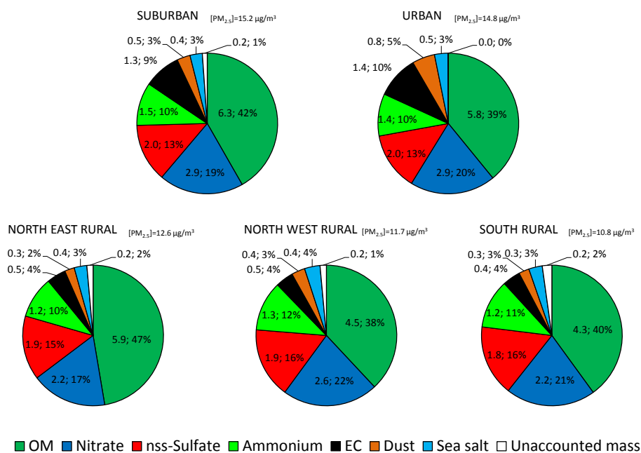
Fig. 9. Annual average chemical composition of PM 2.5 (µg m -3 ; %) at the five sites from 11 September 2009 to 10 September 2010.
