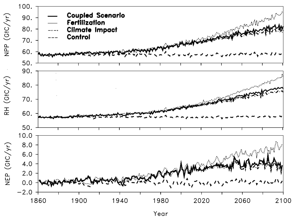
Figure 3. Time series of net primary production (NPP), heterotrophic respiration (RH), and net land carbon uptake (NEP) (in Gt C yr -1 ) for the Control simulation (dashed line), the Coupled Scenario simulation (solid line), the Fertilization simulation (dotted line) and the Climate Impact simulation (dash-dotted line).
