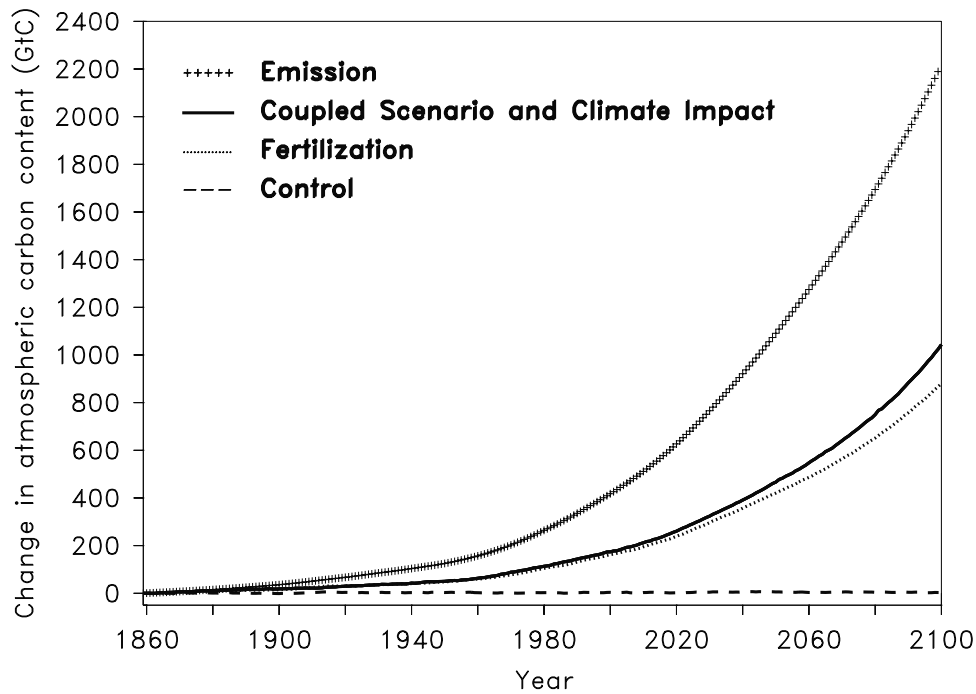
Figure 2. Time series of IPCC/SRES-A2 anthropogenic carbon emissions [Nakicenovic et al., 2000] used as a forcing for the climate model (crosses) and simulated atmospheric carbon content change (departures from preindustrial Holocene) for the Control simulation (dashed line), the Coupled Scenario simulation (solid line) and the Fertilization simulation (dotted line). All numbers are in Gt C.
