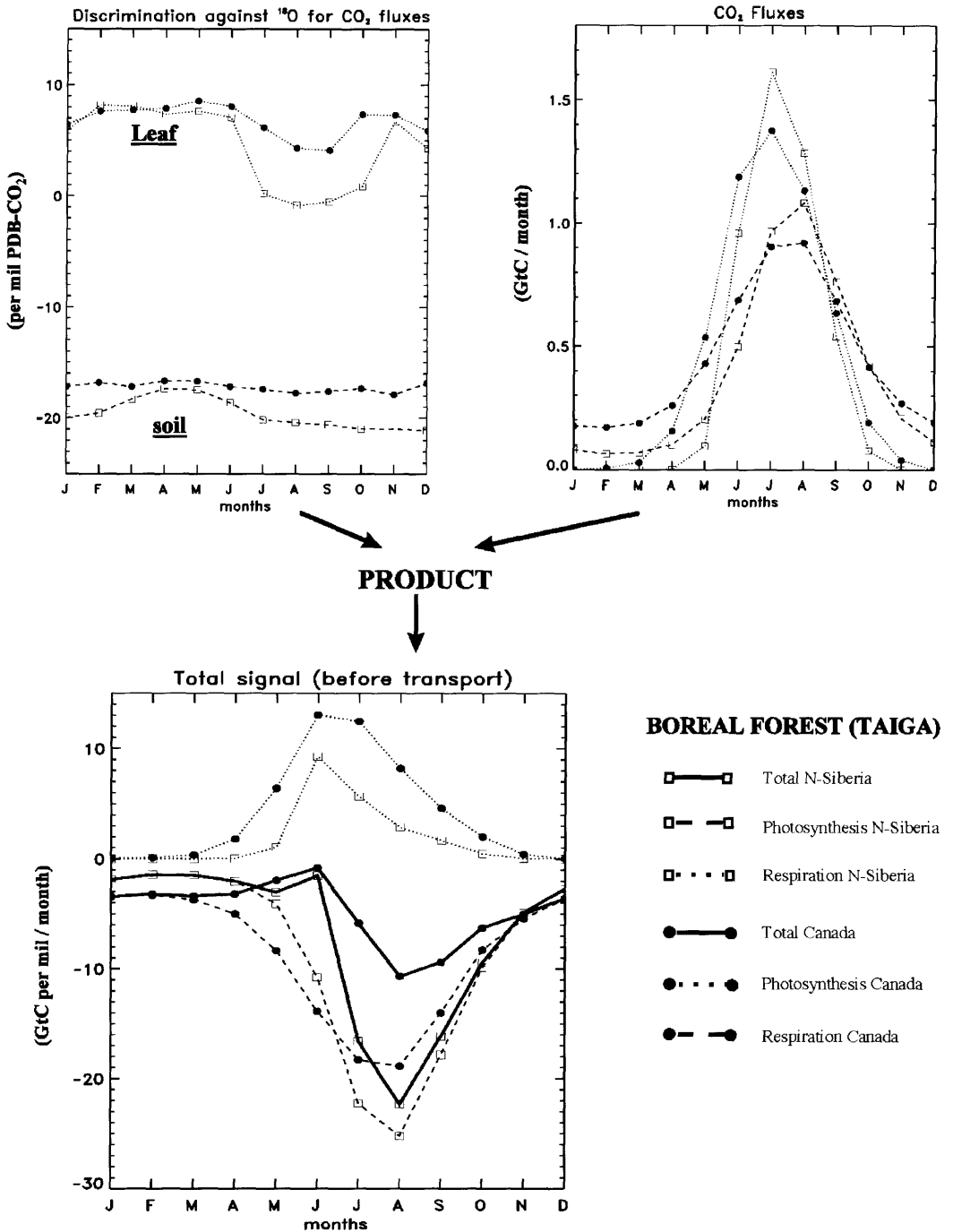
Fig. 9. Seasonal variations of the flux of \delta^{18}\text{O} in atmospheric \text{CO}_2 (in \text{GtC} \cdot \text{month}^{-1} , lower graph) from the northern Siberian taiga and the Canadian taiga (regions 4 and 2, respectively, Fig. 5), before atmospheric transport. The overall contribution (solid lines) is the sum of the photosynthesis and respiration contributions ( A\Delta_A and F_{\text{resp}}\Delta_R , respectively, eq. (A3)), for each region. The isotopic signal from photosynthesis and respiration results from a product between the \text{CO}_2 flux (net assimilation and ecosystem respiration, respectively; upper right graph) and the discrimination against ^{18}\text{O} compared to ^{16}\text{O} associated with this flux (upper left graph).
