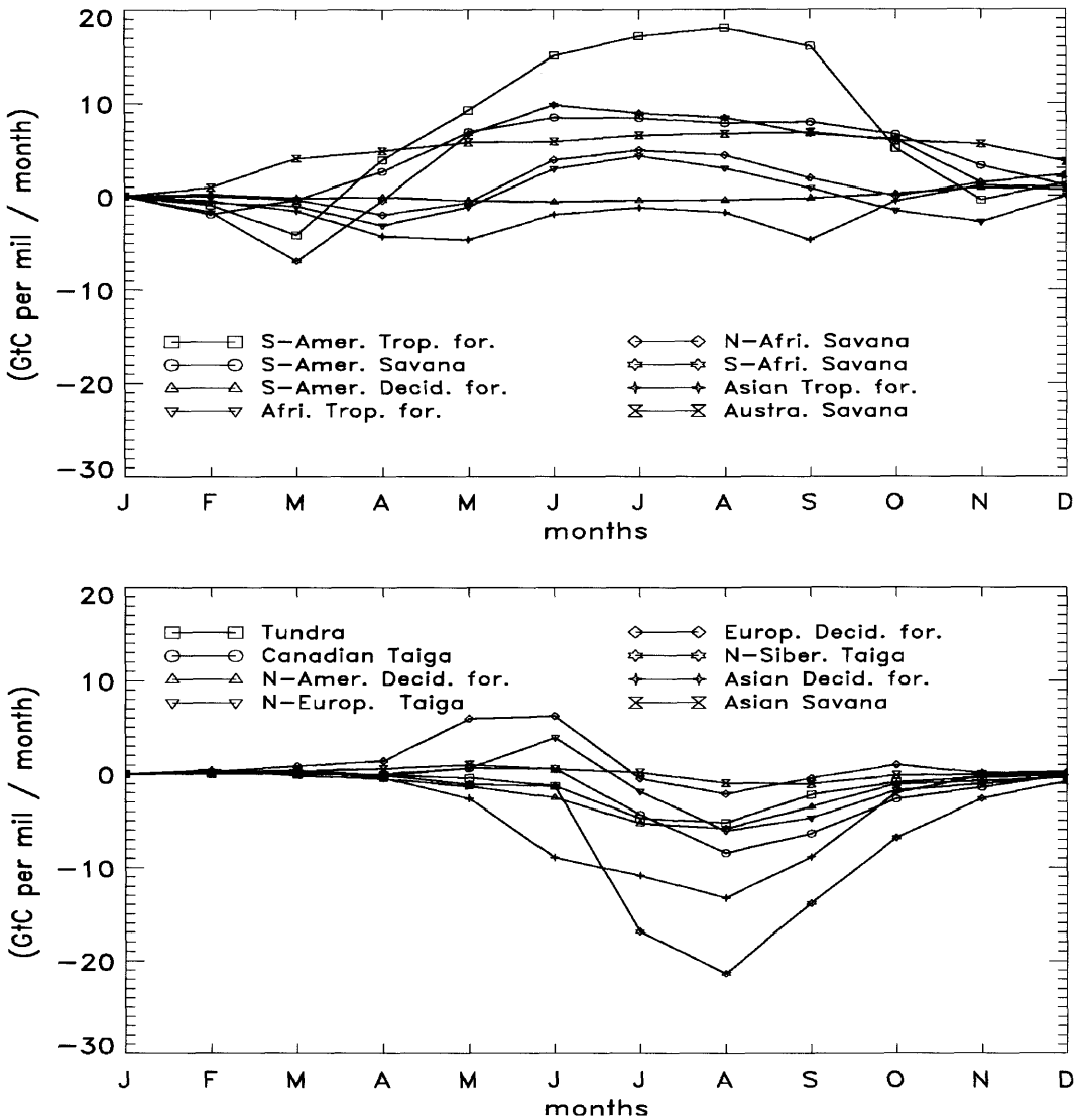
Fig. 8. Seasonal variations of the flux of \delta^{18}\text{O} in atmospheric \text{CO}_2 (in \text{GtC}\% \text{ month}^{-1} ) from 16 land ecosystems (Fig. 5), before atmospheric transport. Values represent the overall contribution of photosynthesis and respiration ( A\Delta_A + F_{\text{resp}}\Delta_R , eq. (A3)). All curves are shifted to zero in January as we will only discuss the seasonality of the fluxes.
