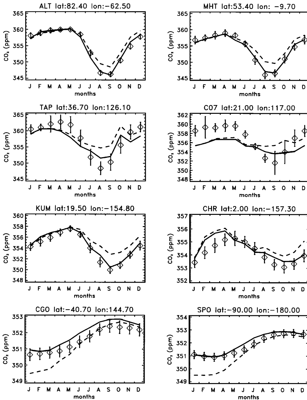
Figure 3. Modeled and observed CO 2 concentrations for 8 of the 77 monitoring sites used in control inversion S_0 . Dots stand for atmospheric data (one climatological year of observations averaging the 1985-1995 period). Dashed line is for the a priori modeled concentrations. Solid line is for the optimized model concentrations.
