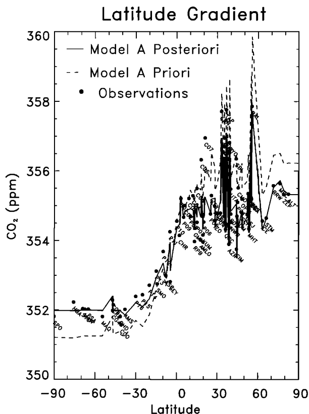
Figure 4. North-to-south gradient. Modeled and observed CO 2 annual concentrations for the 77 monitoring sites used in the control inversion S_0 . Dots stand for atmospheric data (one climatological year of observations averaging the 1985-1995 period). Dashed line is for the a priori modeled concentrations. Solid line is for the optimized model concentrations.
