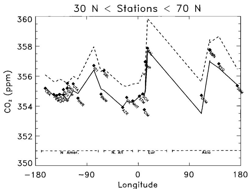
Figure 5. West-to-east gradient. Modeled and observed CO 2 annual concentrations for monitoring sites located between 30°N and 70°N. Dots stand for annual means of atmospheric data (one climatological year of observations averaging the 1985-1995 period). Dashed line is for the a priori modeled concentrations. Solid line is for the optimized model concentrations.
