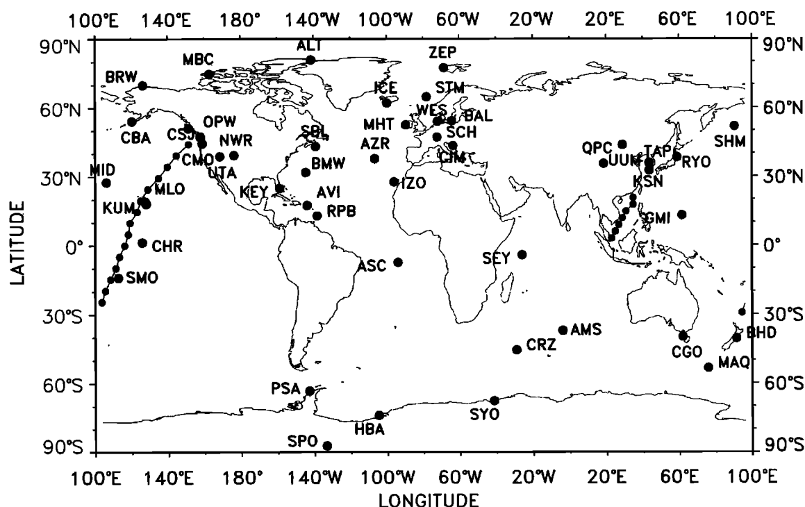
Figure 1. Atmospheric network used for the inverse calculation S_0 . Dots represent ground measurements made by different research groups around the world. Lines represent ship data. Small planes indicates vertical profiles used in the inversion. ALT, Alert; MBC, Mould Bay; ZEP, Spitzberg; BRW, Barrow Point; STM, Station M; ICE, Iceland; CBA, Cold Bay; WES, Westerland; MHT, Mace Head; SHM, Shemya Island; CSJ, Cape S t James; OPW, Olympic Peninsula; SCH, Schauinsland; CMO, Cape Meares; CIM, Monte Cimone; SBL, Sable Island; NWR, Niwot Ridge; UTA, Utah; RYO, Ryori; AZR, Terceira Island; TAP, Tae-ahn Peninsula; QPC, Qinghai Province; KSN, Korean station; BMW, Bermuda West; IZO, Tenerife; MID, Sand Island; KEY, Key Biscayne; KUM, Cape Kumukahi; MLO, Mauna Loa; AVI, S t Croix; GMI, Guam Island; RPB, Ragged Point; CHR, Christmas Island; SEY, Seychelles; ASC, Ascension Island; SMO, American Samoa; AMS, Amsterdam Island; CGO, Cape Grim; BHD, Baring Head; CRZ, Crozet Island; MAQ, Maquarie; PSA, Palmer Station; MAW, Mawson; SYO, Syowa; HBA, Halley Bay; SPO, South Pole; P01 to P16, Pacific cruises; C01 to C07, China Sea cruises; S02 to S06, Aircraft measurements above Japan; CG4 and CG6, Aircraft measurements above Tasmania.
