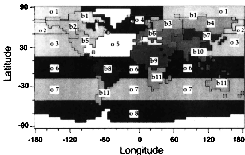
Figure 2. Oceanic (o 1 to o 8) and continental (b1 to b11) regions used by the control inversion S_0 : b1, Arctic (north of 65°N); b2, Boreal North America; b3, Boreal Europe; b4, Boreal Asia; b5, Temperate North America; b6, Temperate Europe; b7, temperate Asia; b8, tropical South America; b9, tropical Africa; b10, tropical Asia; b11, southern nontropical hemisphere; and o 1, north of 65°N; o 2, North Pacific; o 3, far North Atlantic; o 4, North Atlantic; o 5, equatorial oceans, o 6, subantarctic and subtropical oceans; o 7, austral ocean (south of 50°S).
