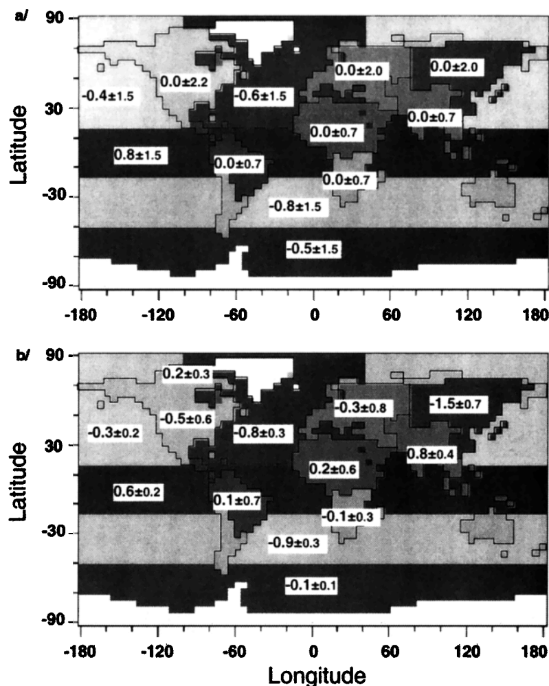
Figure 6. Annual CO 2 net fluxes at continental and ocean basin scale. (a) a priori net fluxes and (b) a posteriori net fluxes inferred in the control inversion S_0 . Fluxes and errors are expressed in Gt C yr -1 .
