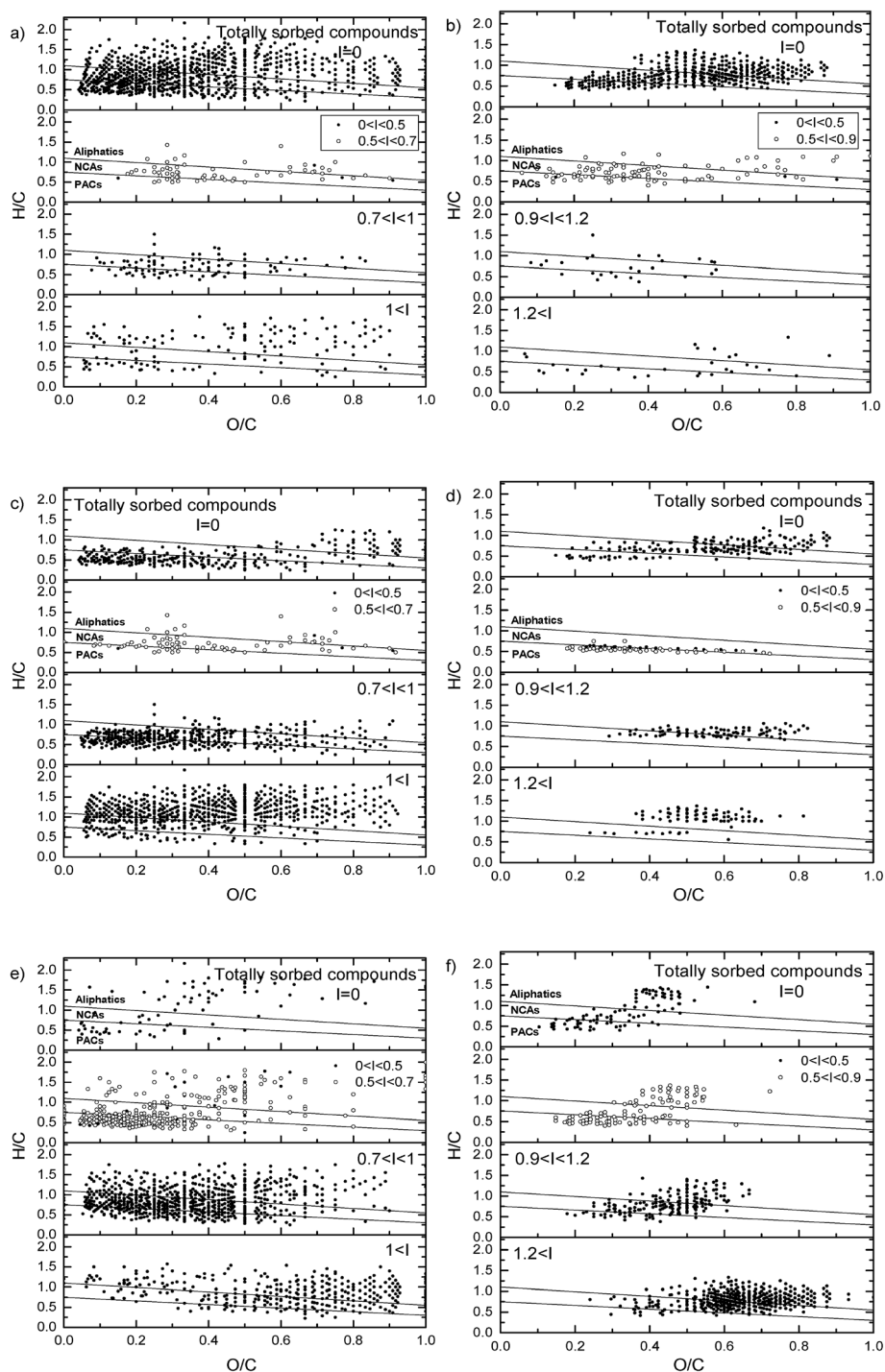
Fig. 3 VK diagrams for PPH compounds sorted as a function of their relative affinities at pH 3.9 for the surface of hematite at r = 0.1 \text{ mg C per m}^2 (a, b), r = 0.6 \text{ mg C per m}^2 (c, d), and r = 1.4 \text{ mg C per m}^2 (e, f) and identified in the mass ranges 120–400 m/z and 400–798 m/z , respectively.
