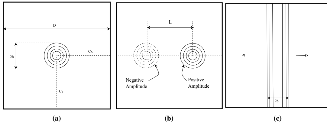
Fig. 3 Schematic of the three test cases. Domain size is D \times D . (a) propagation of single Gaussian Pulse of half-width b , (b) Two Pulses with opposed initial amplitudes and (c) Plane wave with Gaussian profile propagating in x-direction.
