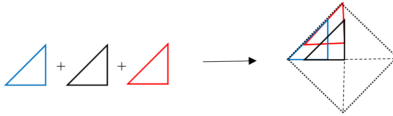
Figure 8 (right isosceles triangles)
