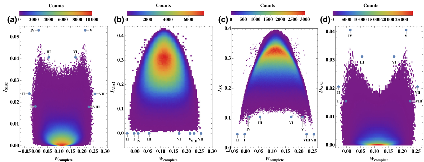
FIG. 6. Histograms of the mutual information and quantum discord versus the total work W_{\text{complete}} . From left to right: (a) I_{S_1S_2} , (b) I_{A_1A_2} , (c) I_{AS} , and (d) D_{S_1S_2} (see definition in the main text). The blue dots are obtained for noncorrelating unitaries specified by their label I–VIII.
