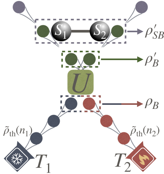
FIG. 1. Setup of our scheme: thermal particles emerging from the cold and hot baths and prepared in the states \tilde{\rho}_{\text{th}}(n_1) and \tilde{\rho}_{\text{th}}(n_2) , respectively, are made to collide to each other under a unitary operation U . The emerging correlated particles in the global state \rho'_B collide with the system's particles S_1 and S_2 .
