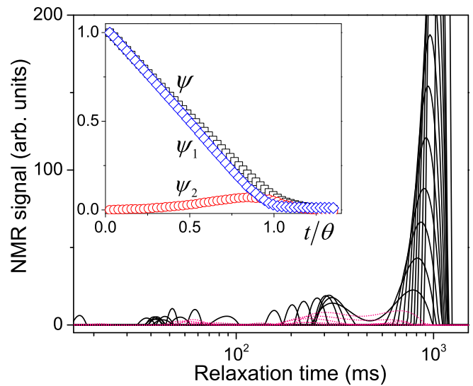
FIG. 6. Drying of a large connected pore medium [see Fig. 2(e) for an illustration]: relaxation time distributions at different successive times (every 7 min) (from right to left) during drying, first as black continuous lines, then as pink dotted lines from the last distribution reflecting liquid in large pores. For the sake of clarity only one in three measured distributions is represented. The inset shows the liquid fractions of the different regions (black squares for the total liquid fraction, blue diamonds for the liquid fraction in large pores, red circles in small pores) as a function of the dimensionless time ( \theta = 5350 s).
