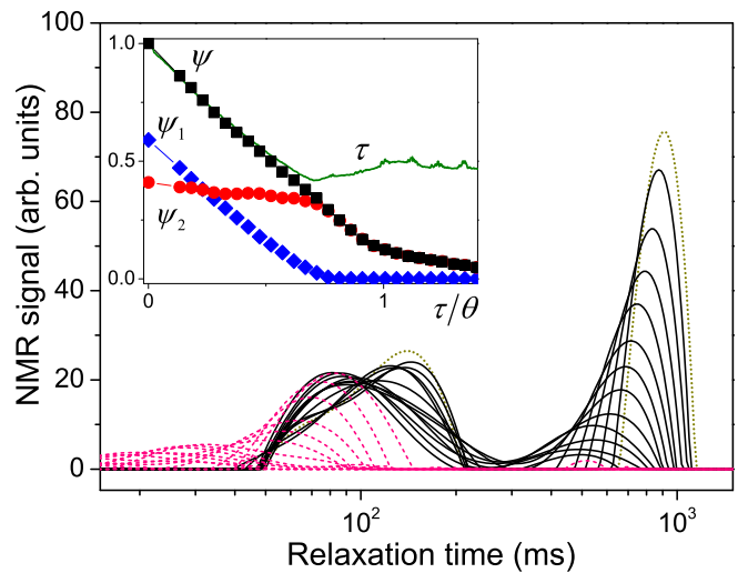
FIG. 8. Drying of a biporous medium [ n = 0.59 , see Fig. 2(c) for an illustration]: relaxation time distributions at different successive times (every 13 min) (from right to left) during drying, first as black continuous lines, then as pink dashed lines from the last distribution reflecting liquid in large pores. The initial curve is drawn as a dotted line. The inset shows the liquid fractions of the different regions (black squares for the total liquid fraction, blue diamonds for the liquid fraction in large pores, red circles in small pores) and the liquid-phase contraction rate (green continuous line) as a function of the dimensionless time ( \theta = 17800 s).
