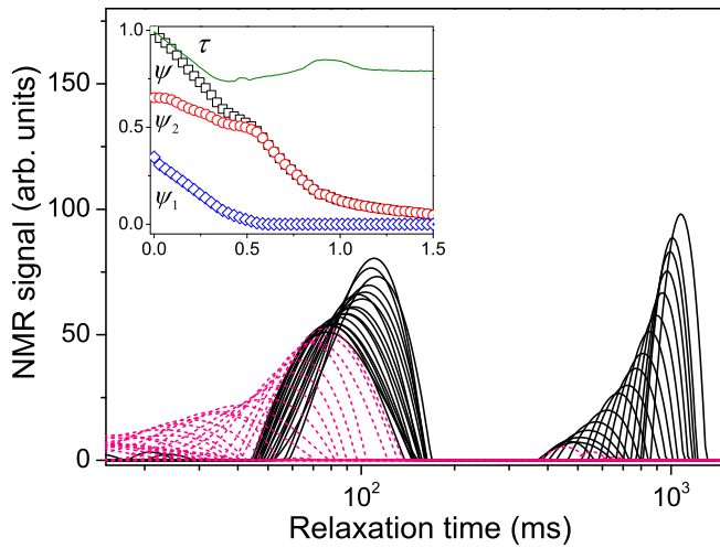
FIG. 9. Drying of a biporous medium [ n = 0.34 , see Fig. 2(b) for an illustration]: relaxation time distributions at different successive times (every 14.5 min) (from right to left) during drying, first as black continuous lines, then as pink dashed lines from the last distribution reflecting liquid in large pores. The inset shows the liquid fractions of the different regions (black squares for the total liquid fraction, blue diamonds for the liquid fraction in large pores, red circles in small pores) and the liquid-phase contraction rate (green continuous line) as a function of the dimensionless time ( \theta = 28400 s).
