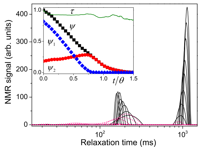
FIG. 7. Drying of a connected biporous system [see Fig. 2(d) for an illustration]: relaxation time distributions at different successive times (every 25 min) (from right to left) during drying, first as black continuous lines, then as pink dashed lines from the last distribution reflecting liquid in large pores. For the sake of clarity only one of the two measured distributions is presented. The inset shows the liquid fractions of the different regions (black squares for the total liquid fraction, blue diamonds for the liquid fraction in large pores, red circles in small pores) and the liquid-phase contraction rate (green continuous line) as a function of the dimensionless time ( \theta = 16150 s).
