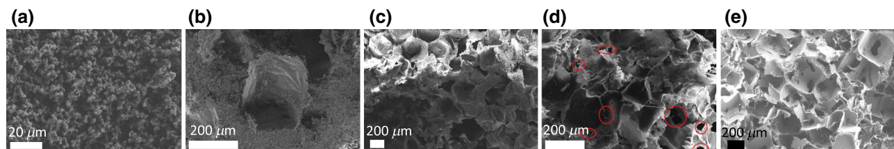
FIG. 1. Images of the different system types obtained from scanning electron microscopy: (a) microporous; (b) nonconnected biporous ( n = 0.24 ), (c) nonconnected biporous ( n = 0.59 ), (d) connected biporous ( n = 0.81 ), (e) macroporous. Red contours in (d) indicate interconnections between large pores. These interconnections are more directly visible (black holes) in (e).
