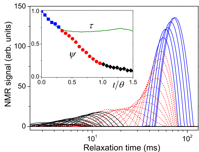
FIG. 5. Drying of a homogeneous medium with small pores [see Fig. 2(a) for an illustration]: relaxation time distributions at different successive times (every 21 min) (from right to left) during drying. The inset shows the liquid fraction and the liquid-phase contraction rate as a function of the dimensionless time ( \theta = 22100 s). Three regimes are identified: sample contraction (blue continuous lines and squares), homogeneous air penetration (red dashed line and circles), dry front development (black continuous lines and diamonds).
