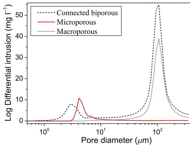
FIG. 12. Mercury porosimetry intrusion profiles for different samples (data from [22]).
