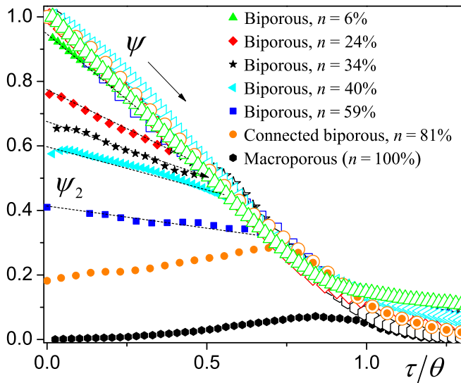
FIG. 11. Total liquid fraction (open large symbols) and liquid fraction in small pores (small filled symbols) and saturation in small pores times the initial fraction of small pores (small filled symbols) as a function of the rescaled time during drying for the different dispersed biporous structures (i.e., unconnected large pores), the connected biporous structure and the macroporous structure.
