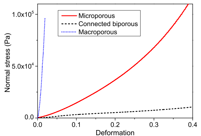
FIG. 3. Normal stress versus deformation during a compression test for different sample types.
