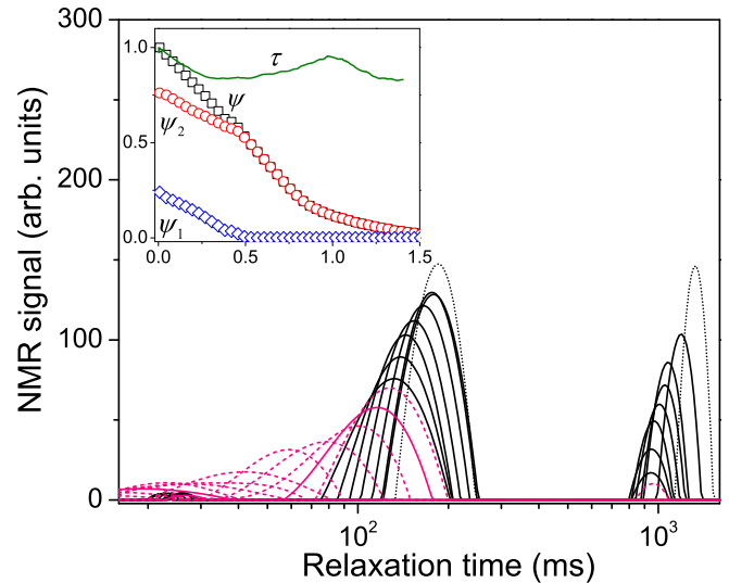
FIG. 10. Drying of a biporous medium [ n = 0.24 , see Fig. 2(b) for an illustration]: relaxation time distributions at different successive times (every 14.5 min) (from right to left) during drying, first as black continuous lines, then as pink dashed lines from the last distribution reflecting liquid in large pores. The initial curve is drawn as a dotted line. For the sake of clarity only one in two distributions is represented except for the two first distributions. The inset shows the liquid fractions of the different regions (black squares for the total liquid fraction, blue diamonds for the liquid fraction in large pores, red circles in small pores) and the liquid-phase contraction rate (green continuous line) as a function of the dimensionless time ( \theta = 20700 s).
