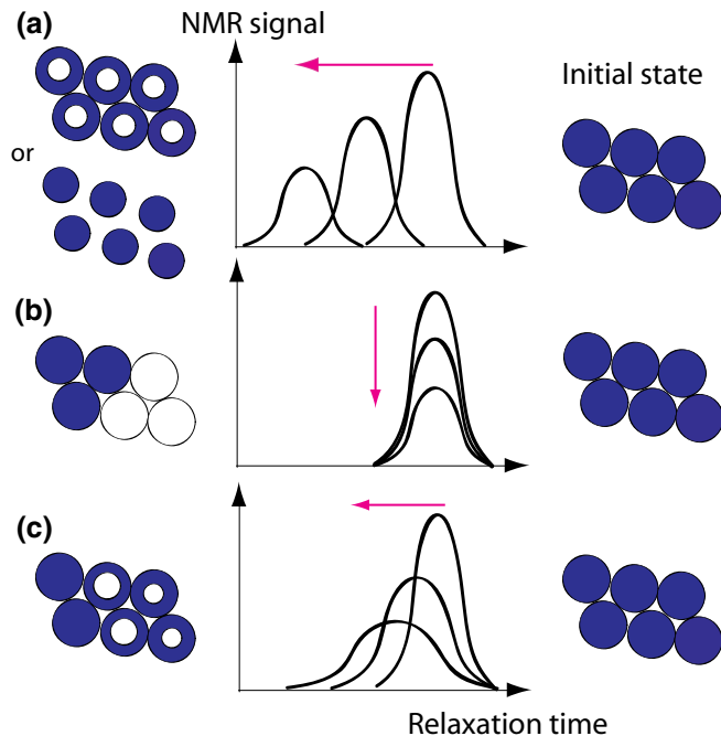
FIG. 4. Evolution of the T distribution in different ideal cases of water extraction from pores [disks initially filled with water (in blue)]: (a) homogeneous pore shrinkage or pore desaturation, (b) heterogeneous pore emptying, (c) heterogeneous pore desaturation.
