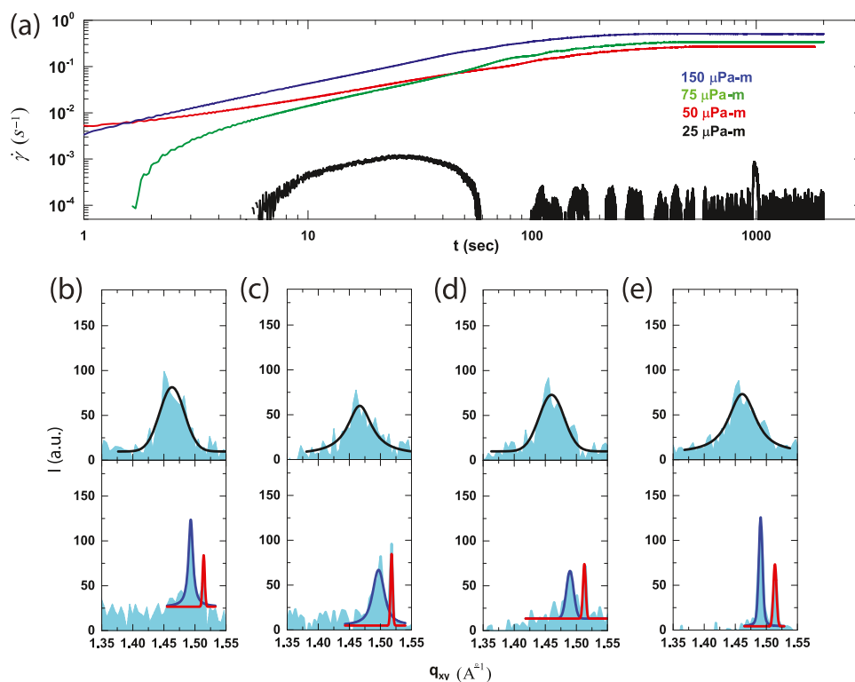
Figure 6. Rheo-GIXD creep data of the DPPC–alamethicin mixed monolayer with the molar ratio P/L = 1:2 (presheared for 200 s followed by a waiting time of 300 s before each measurement; see text): (a) creep curves; \dot{\gamma} vs t are plotted. Bragg peaks q_{02} (blue solid fit) and q_{11} (black solid fit) and the alamethicin helix peak (red solid fit) for different \sigma values of (b) 25 \mu\text{Pa}\cdot\text{m} , (c) 50 \mu\text{Pa}\cdot\text{m} , (d) 75 \mu\text{Pa}\cdot\text{m} , and (e) 150 \mu\text{Pa}\cdot\text{m} are shown. The peaks are fitted using a Voigt function.
