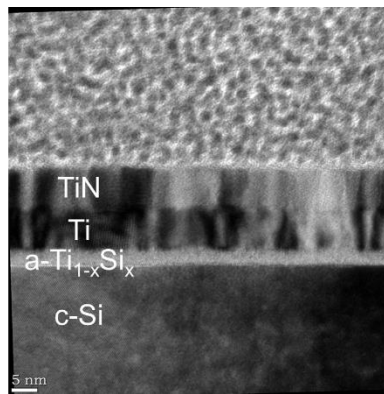
Fig. 1 – TEM micrograph corresponding to the as-deposited sample TiN/Ti/Si. The TiN and Ti target thicknesses were fixed around 10 nm. Three layers are clearly identified as TiN, Ti and a\text{-Ti}_{1-x}\text{Si}_x on top of the Si substrate.
