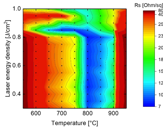
Fig. 8 - 2D color map showing the evolution of R_s for TiN/Ti/Si samples first exposed to 3 UV-NLA pulses at ED in the 0.30\text{-}1.00 \text{ J}/\text{cm}^2 range (Y axis) and submitted to RTA in the 550\text{-}900^\circ\text{C} range (X axis). Black dots in 2D map are the measured data points.
