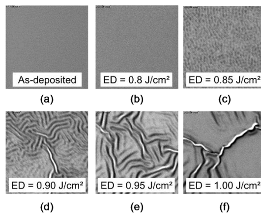
Fig. 7 - 5 \times 5 \mu\text{m}^2 top-view SEM observations of TiN/Ti/Si samples (a) as-deposited or submitted to 3 UV-NLA pulses with following laser ED : (b) 0.80, (c) 0.85, (d) 0.90, (e) 0.95 and (f) 1.00 \text{J/cm}^2 .
