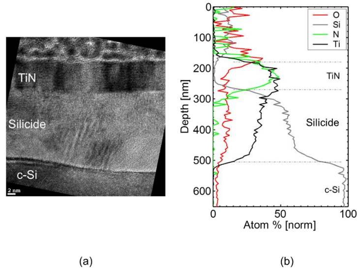
Fig. 5 - (a) HRTEM micrograph corresponding to the sample annealed at 0.85 \text{ J/cm}^2 with 3 UV-NLA pulses. TiN and Ti-silicide layers are clearly identified on top of the Si substrate. (b) TEM-EDX depth profiles for the same sample.
