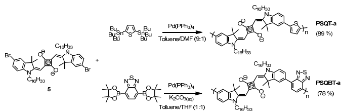
Scheme 2 Syntheses of Poly(squaraine- alt -thiophene) and poly(squaraine- alt -benzothiadiazole) via Suzuki and Stille cross-coupling.
