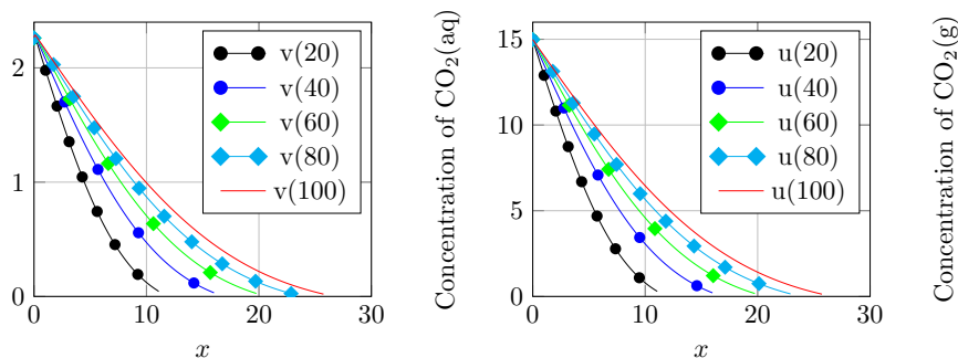
Figure 1: Profiles of v (on the left) and u (on the right) at different times. The solutions are plotted on [0, s(t)] .
