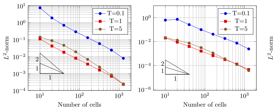
Figure 4: L^2 -norm of the error for u (on the left) and v (on the right) in space at different final times with the upwind fluxes.
