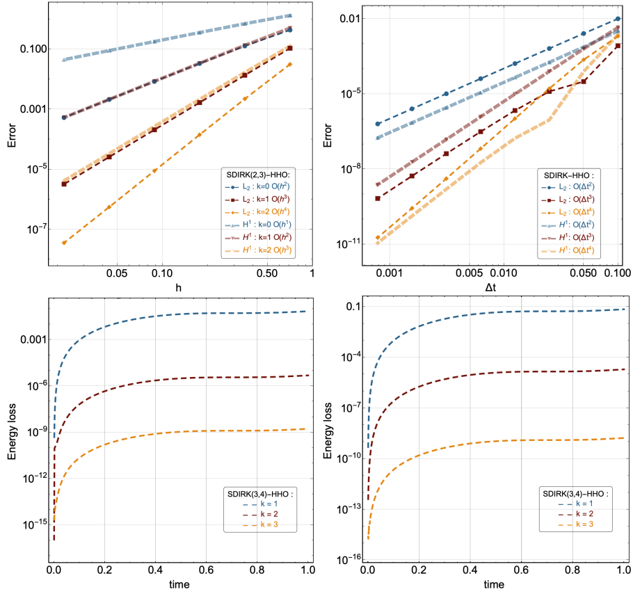
Figure 2: HHO-SDIRK( s, s+1 ), equal-order case. Top row: errors as a function of the mesh-size for the analytic solution (78) (left panel, s=2 ) and as a function of the time-step for the analytic solution (79) and k=2 (right panel, s \in \{1, 2, 3\} ). Bottom row: relative energy loss as a function of time for the analytical solution is (80) in the equal-order (left panel) and mixed-order (right panel) cases with s=3 , h=2^{-5} , and \Delta t=0.1 \times 2^{-7} .
