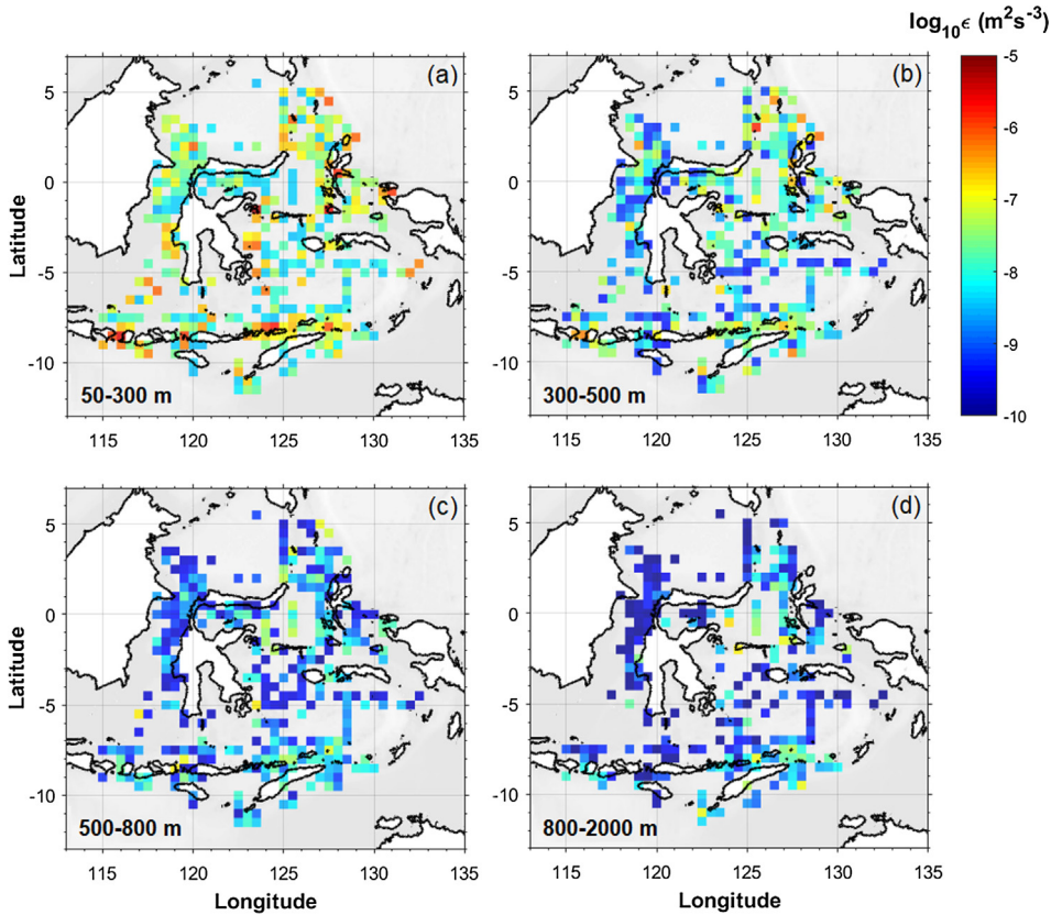
Fig. 1. A half degree grid mean of turbulent kinetic energy dissipation rates ( \epsilon , in \log_{10} \text{ m}^2\text{s}^{-3} ) inferred from geographically distributed historical CTD datasets using improved Thorpe method proposed by Purwandana et al. [1] at (a) 50–300 m, (b) 300–500 m, (c) 500–800 m, (d) 800–2000 m.
