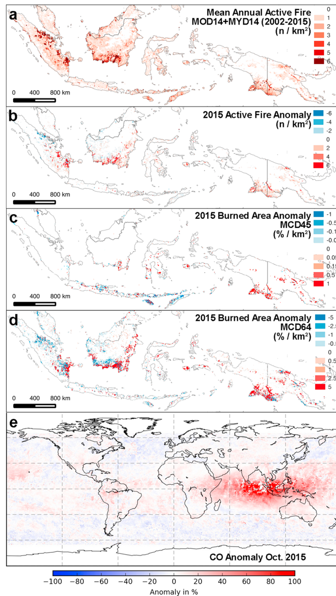
Figure 2. Spatial distribution of fire anomaly in 2015. (a) Mean annual active fire counts from both the morning (MOD14) and the afternoon (MYD14). (b) Active fire anomaly. (c) Burned area anomaly in MCD45 compared to its multiyear average (2003–2015). (d) Burned area anomaly in MCD64 compared to its multiyear average (2003–2015). (e) MOPITT X_{CO} anomaly in October 2015 compared to its multiyear October average (2002–2015).
