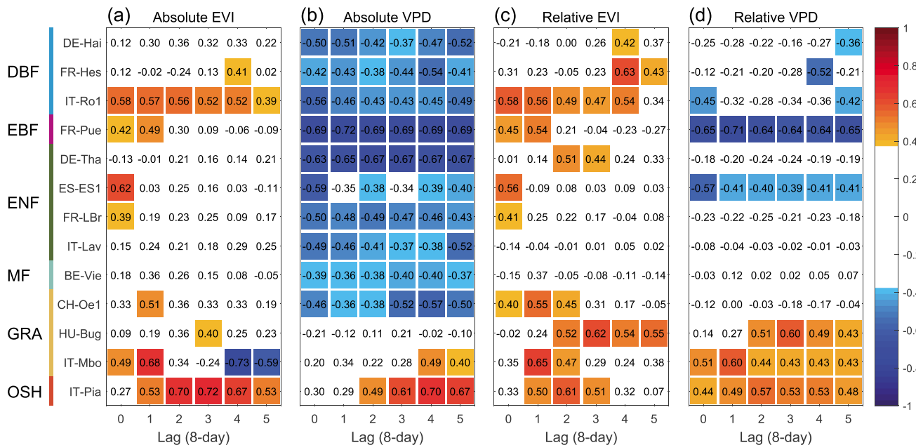
Figure 2. Partial correlation between anomalies in GPP and anomalies in (a and c) EVI and (b and d) VPD. EVI with different lags were used. Figures 2a and 2b are using absolute anomalies ( \Delta_y ) and Figures 2c and 2d are using relative anomalies ( \sigma_y ). Only partial correlations that are significant at 0.1 level ( p < 0.1 ) are shown in reddish or bluish color. The numbers represent the partial correlation coefficients.
