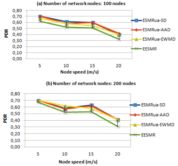
Fig. 4. PDR versus node speed (for manhattan model). The PDR (Packet delivery ratio) is shown in Fig. 4 with different number of network nodes for various moving speeds. The PDR of ESMRua for three variants of calculating coefficient of variation is higher than EESMR for manhattan model. Our protocol successfully receives more packets compared to EESMR protocol mainly for a medium or high number of network nodes, which ensures a good reliability of our protocol for not-random models of mobility designed for cities. ESMRua selects the best paths in term energy, stability and signal quality.
