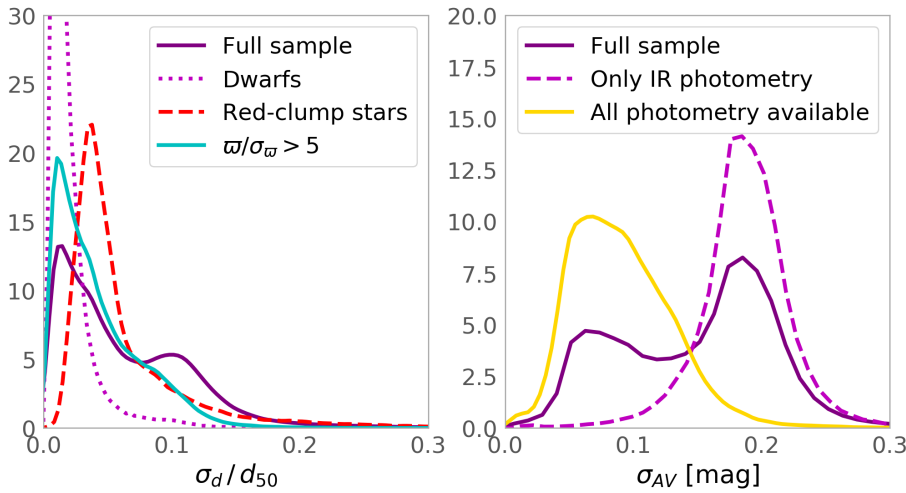
Fig. 4. Kernel-density estimates of the uncertainty distributions for the distances (left panel) and A_V extinctions (right panel) in the APOGEE DR16 StarHorse VAC. The different curves show the distributions of distances and extinctions uncertainties for subsets of different data input quality. Left panel: we highlight the higher distance precision achieved for a stars with Gaia DR2 parallaxes more precise than 20%, b dwarf stars ( \log g < 4 ), and c red-clump stars ( 2.3 < \log g < 2.5 ). In the right panel, we show how the (un-)availability of optical photometry drastically improves or worsens the precision of our A_V estimates.
