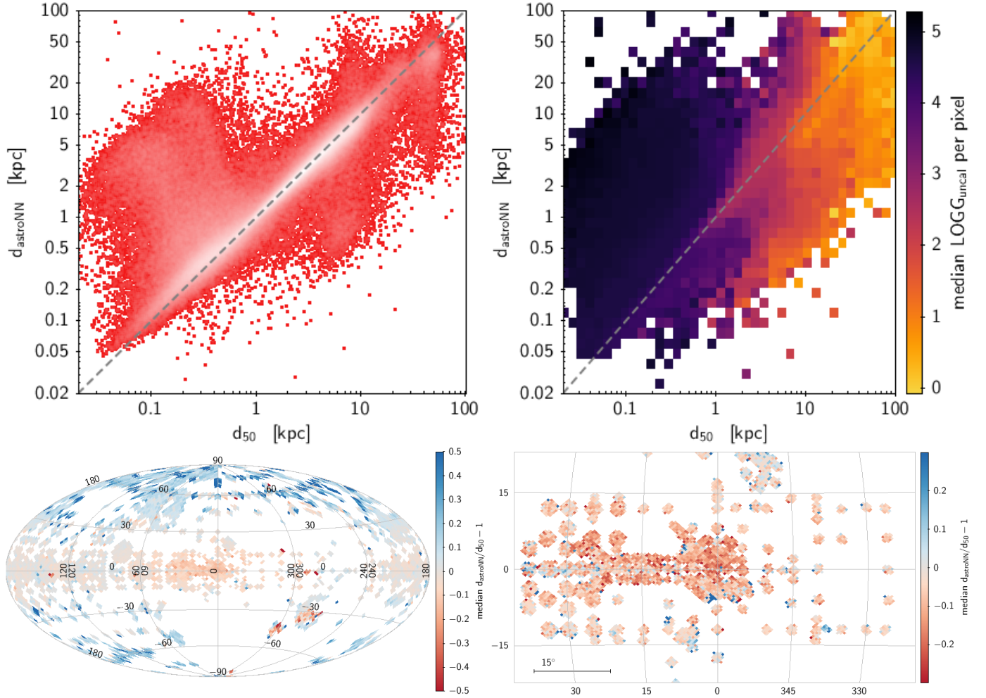
Fig. B.6. Comparison with astroNN distances presented by Leung & Bovy (2019) . Top panel: 1-to-1 comparison ( left: density distribution; right: colour-coded by median uncalibrated surface gravity determined by ASPCAP, showing that astroNN is overestimating distances to dwarf stars). Bottom panels: relative distance differences as a function of sky position ( left: whole sky, right: zoom into the inner Galaxy).
