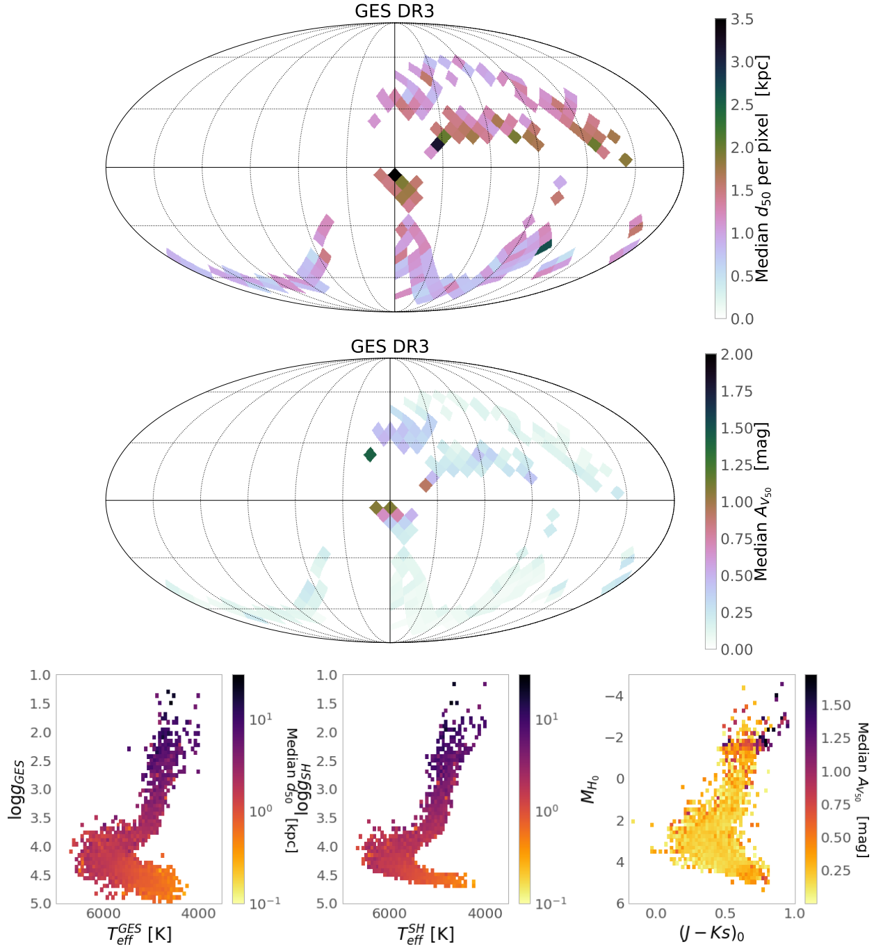
Fig. C.4. Similar to Figs. 2 and 3, but for GES DR3 data.
