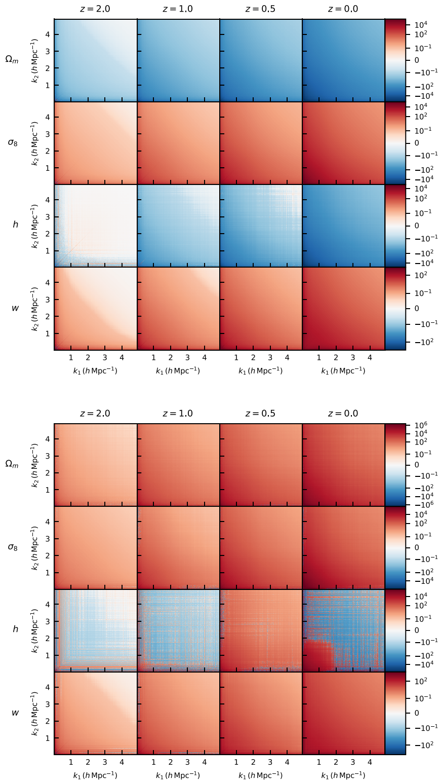
Figure 2. First (top) and second (bottom) derivative of the covariance with respect to \Omega_m (first row), \sigma_8 (second row), h (third row), and w (fourth row). The columns from left to right corresponds to redshift z = 2, 1, 0.5 , and 0 , respectively.
