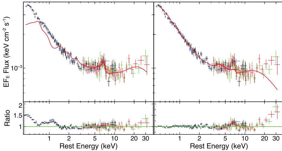
Figure 8. The 2016 XMM-Newton and NuSTAR spectra of Ton S180 fitted with relxill where the overall model (solid red line) is overlaid to the data. Left: fit in the 3–30 keV energy range where the Fe K profile and the hard X-ray data are well reproduced. However, the extrapolation down to 0.4 keV of the model fails to account for the soft excess leaving strong residuals below 2 keV. Right: fit in the 0.4–30 keV energy band. While the soft excess is now well accounted for, the model cannot adequately fit the Fe K emission nor the hard X-rays at E > 10 keV. Fitting the XMM-Newton and NuSTAR spectra with a standard reflection model cannot account self-consistently for the soft and hard X-ray bands. The values for both cases are tabulated in Table 3.
