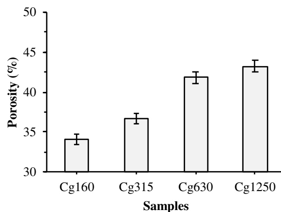
Figure 5. Porosity of samples.
