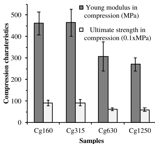
Figure 12. Compression modulus of elasticity and maximum stress of samples.
