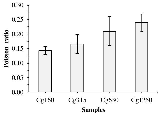
Figure 10. Poisson's ratio of samples.
