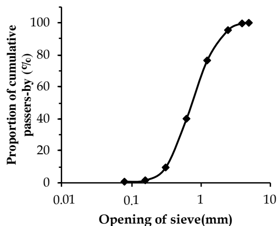
Figure 1. Grain size curve of sawdust used.
