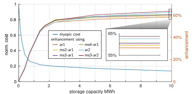
Fig. 8: Left axis: Normalized operating costs depending on battery size with myopic control – in blue. Right axis: Relative enhancement versus myopic control.
