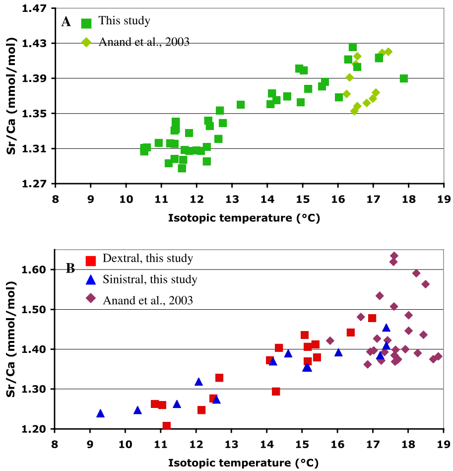
Figure 10. Plot showing mean Sr/Ca ratio and Tiso obtained from (a) G. inflata and (b) G. truncatulinoides from core tops (this study) and measurements from the sediment trap samples [ Anand et al. , 2003] for these species.
