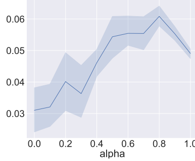
Fig. 6: Mean WRAcc vs \alpha
