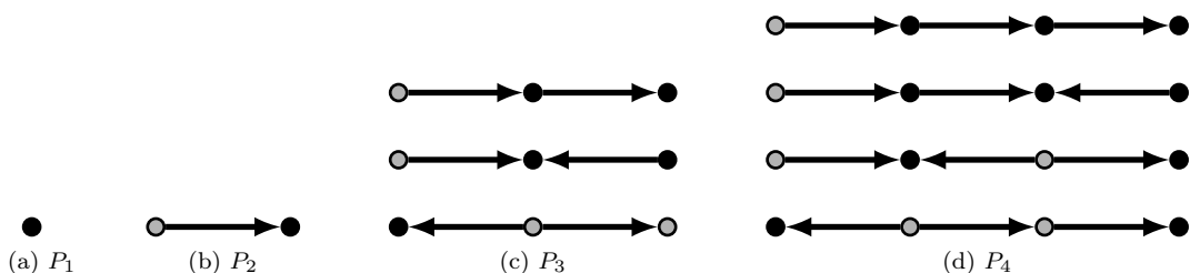
Figure 2: Non-isomorphic orientations of P_n for n \in \{1, 2, 3, 4\} . For each orientation, the set of grey vertices is a minimum resolving set.
