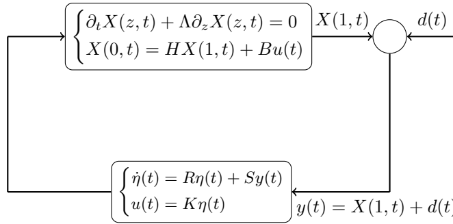
Fig. 3: Control architecture used for stabilization of hyperbolic system in the presence of disturbances.
