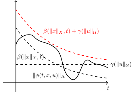
(b) Typical solution of an ISS system with u \neq 0
