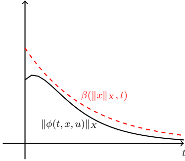
(a) Typical solution of an ISS system with u \equiv 0
