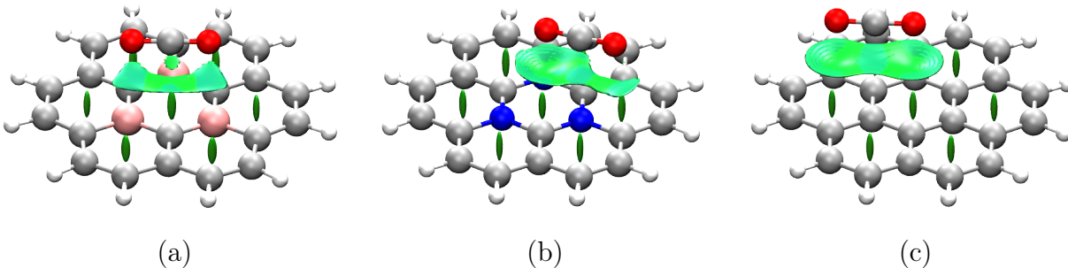
Figure 10: CO 2 adsorption on top of different graphene-like flakes: (a) B-doped graphene (b) N-doped graphene flake (c) non-substituted graphene flake .
