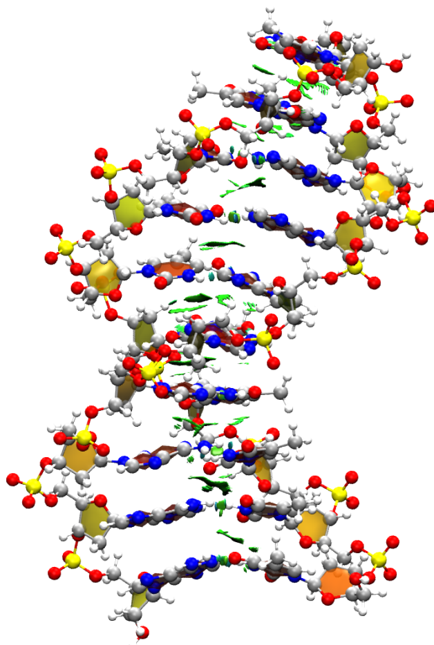
Figure 11: s(\mathbf{r}) = 0.3 isosurface in an intramolecular calculation fo a DNA fragment.
