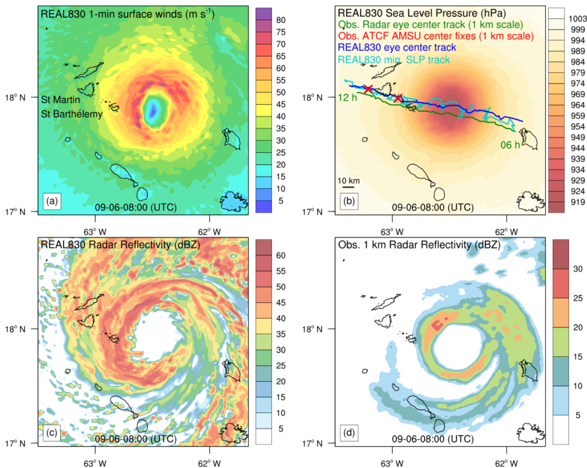
Figure 3: Simulated Irma eye at 830 m scale and at 08:00 UTC (REAL830). (a) Sustained surface winds ( m s^{-1} ). (b) Sea Level Pressure (hPa) with simulated tracks and observed radar eye center track. The time interval for all tracks is 5 minutes. (c) Simulated radar reflectivity (dBZ). (d) Observed radar reflectivity (dBZ).
