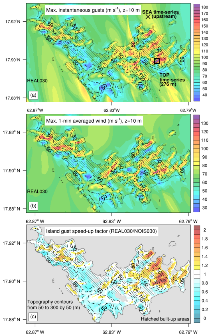
Figure 7: Saint Barthélemy 30-m scale maximum surface winds during the 6 hours of simulation (history output interval of 1 min). (a) Maximum instantaneous gust (m s -1 ) with locations of two numerical time-series stations: SEA and TOP. (b) Maximum 1-min averaged wind in m s -1 . (c) Island gust speed-up factor (REAL030/NOIS030). Topography contours in m and hatched built-up areas are plotted on the three panels.
