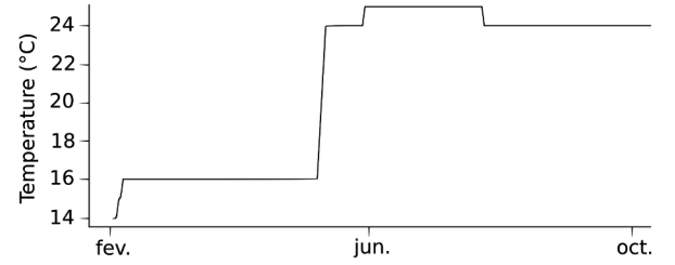
Fig. 3. Temperatures experienced by young seabass in the experiment of Allal et al. (unpublished) and used to validate our DEB model with an independent dataset.
