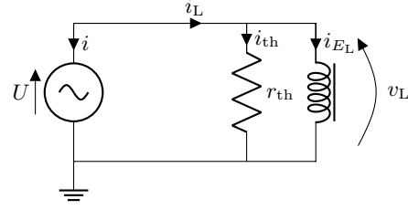
Figure 4: Voltage-controlled ferromagnetic coil with thermal dissipation.
