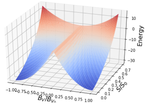
Figure 1: Core energy function with respect to B_V and S .
