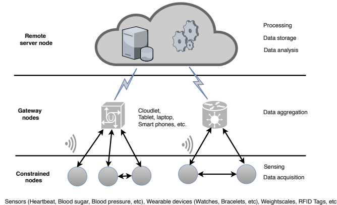
Figure 1: Network Model
