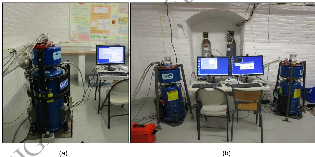
Figure A2. Measuring setup for iGrav023 (a) and iGrav032 and iGrav015 (b) at the gravimetric observatory J9 in June 2017; with each instrument connected to a separate helium cooling system and data acquisition unit.
