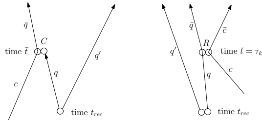
FIGURE 14. The first deflection of q can be either a collision, or a clustering recollision.
